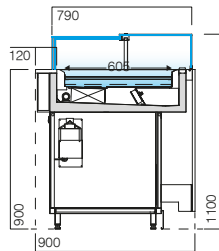
VMIND - VDB UV 3M2/3S dupla temperatura dual-temperature dual-temperature dual-temperature
