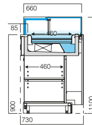
VMINSD - VDB UV 3M2/3S ventilada bitemperatura dual-temperature ventilated ventilée dual-temperature ventilada dual-temperatura
