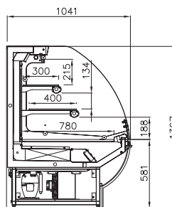
PVM - VCV-CH vitrina mural multideck display murale vitrine vitrina mural
