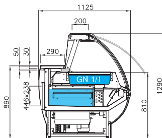
PRSL - VCV-CH 3H saladas salads saladette ensaladas
